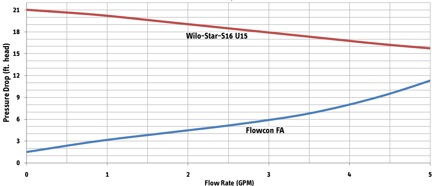
SE Flowstar Pressure Drop Characteristics
